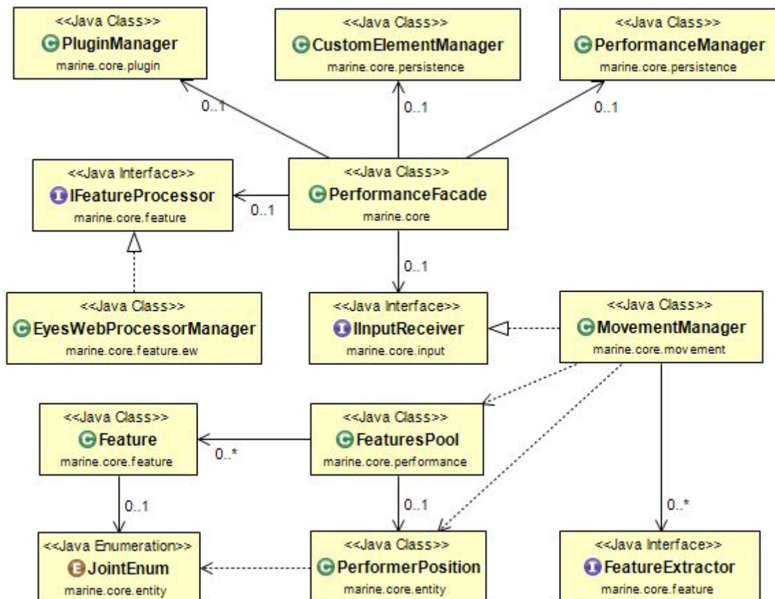
marine core internal modules ("mistic.scholz" omitted on package names)
