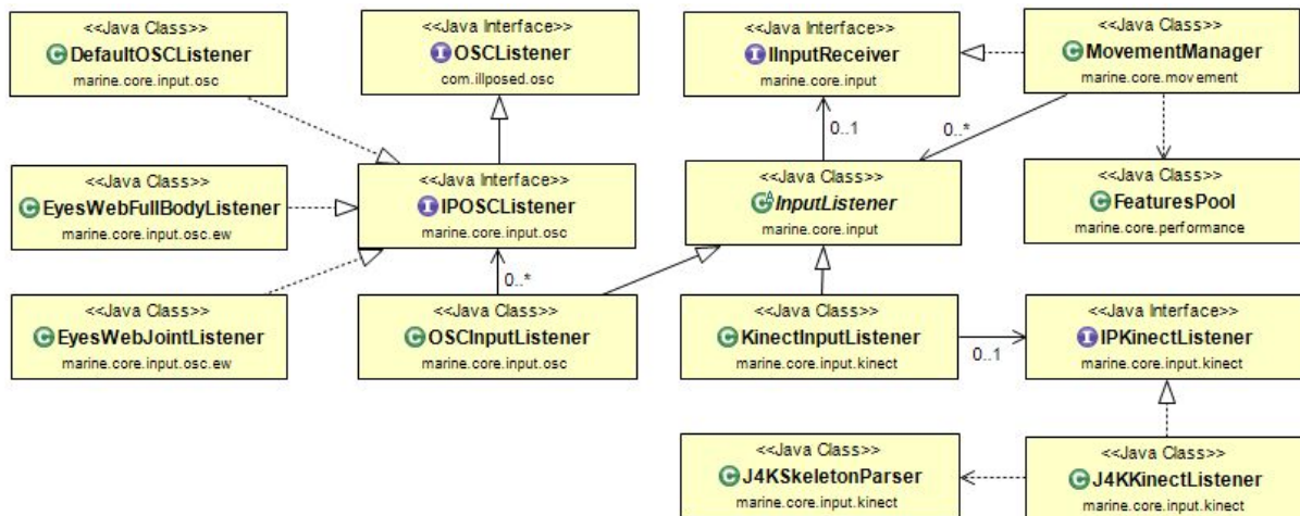
marine Input Listeners Model (“mustic.scholz” omitted on package names)
