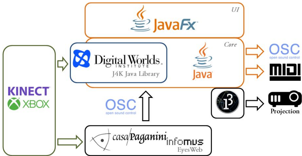
High level architecture organization: marine modules in orange.
